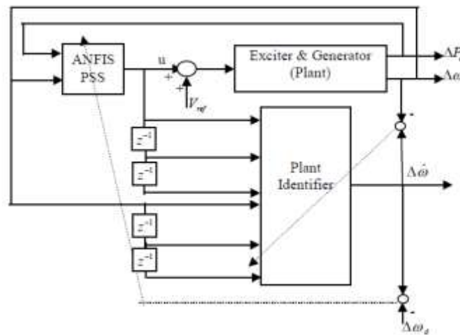
Fig. 1: Structure of Controlled System
