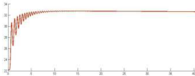
Fig 6 (b): Rotor Angle of Synchronous Generator at Normal Load Condition
