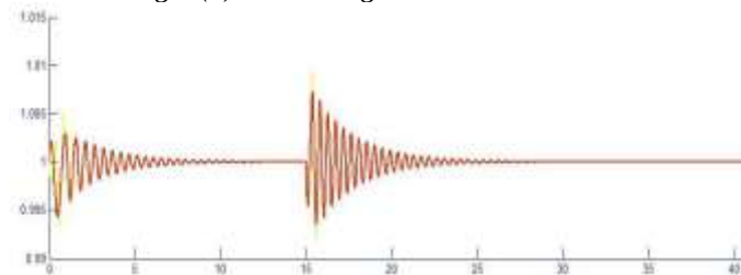
Fig 7 (c): Speed Deviation of Synchronous Generator at Fault Condition
