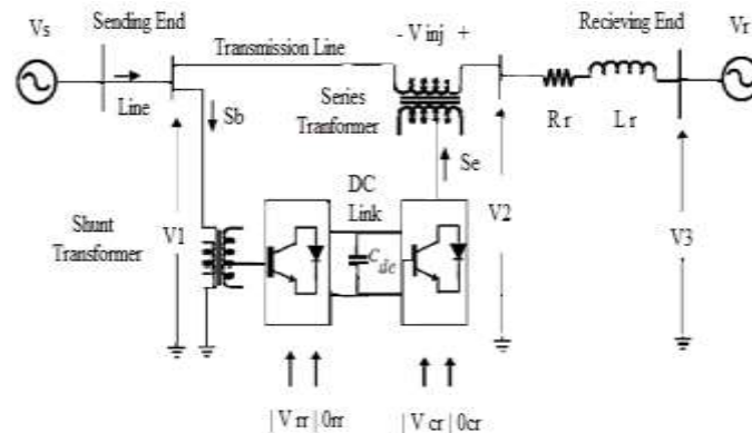
Fig.5: Connection diagram of UPFC with transmission line
