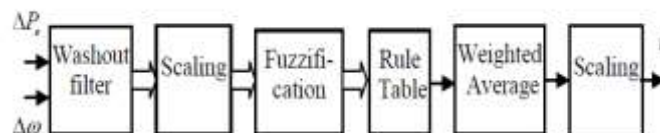
Fig. 2: Block Diagram of ANFIS Model
