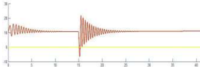
Fig 7 (a): Active Power at Fault Condition
