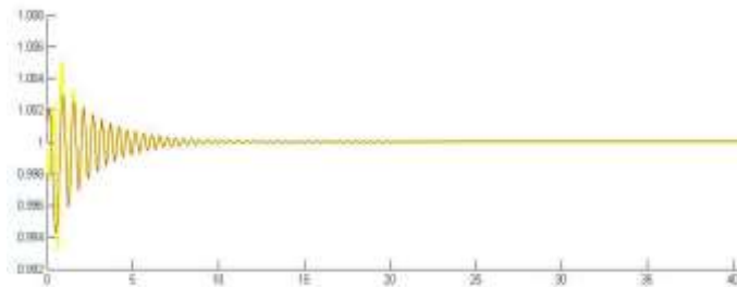
Fig 6 (c): Speed Deviation of Synchronous Generator at Normal Load Condition
