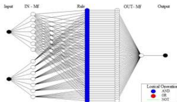
Fig. 3: ANFIS Architecture of PSS Controller
