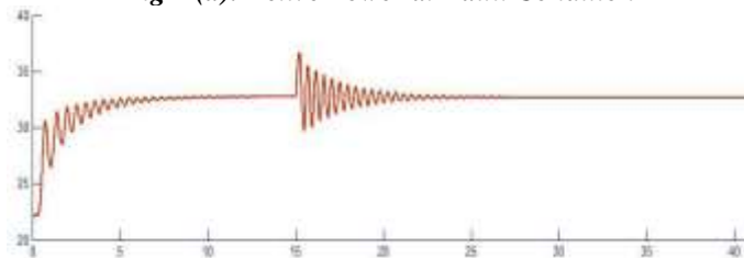
Fig 7 (b): Rotor Angle at Fault Condition
